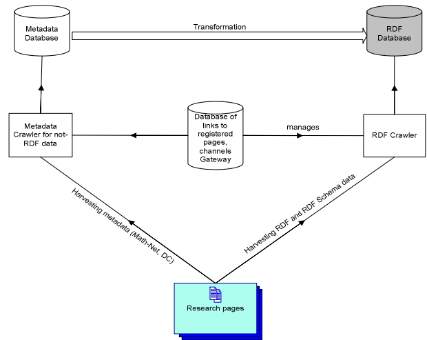
Fig. Metadata collecting into RDF database
