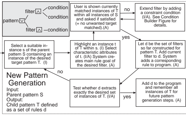
Figure 3: Generation of a new Pattern
