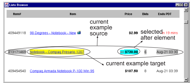
Figure 2: The Lixto Browser
