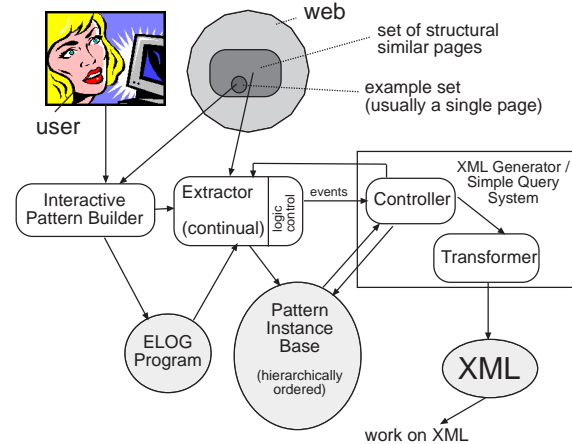
Figure 1: Overview of the Lixto System
