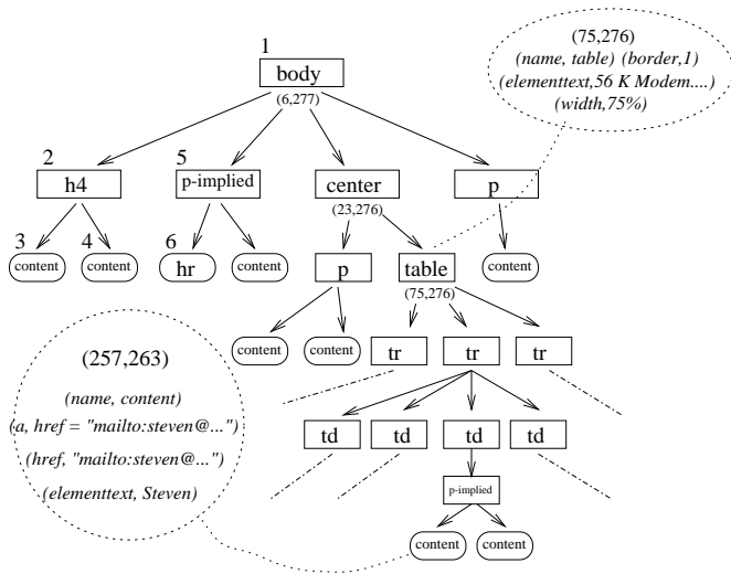
Figure 7: HTML Parse Tree of Example in Figure 6
